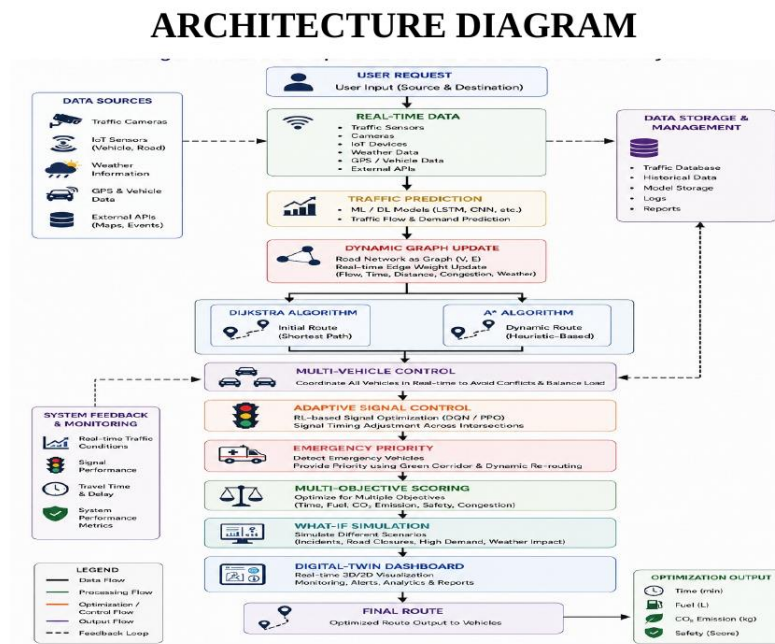
Figure 1. System Architecture
