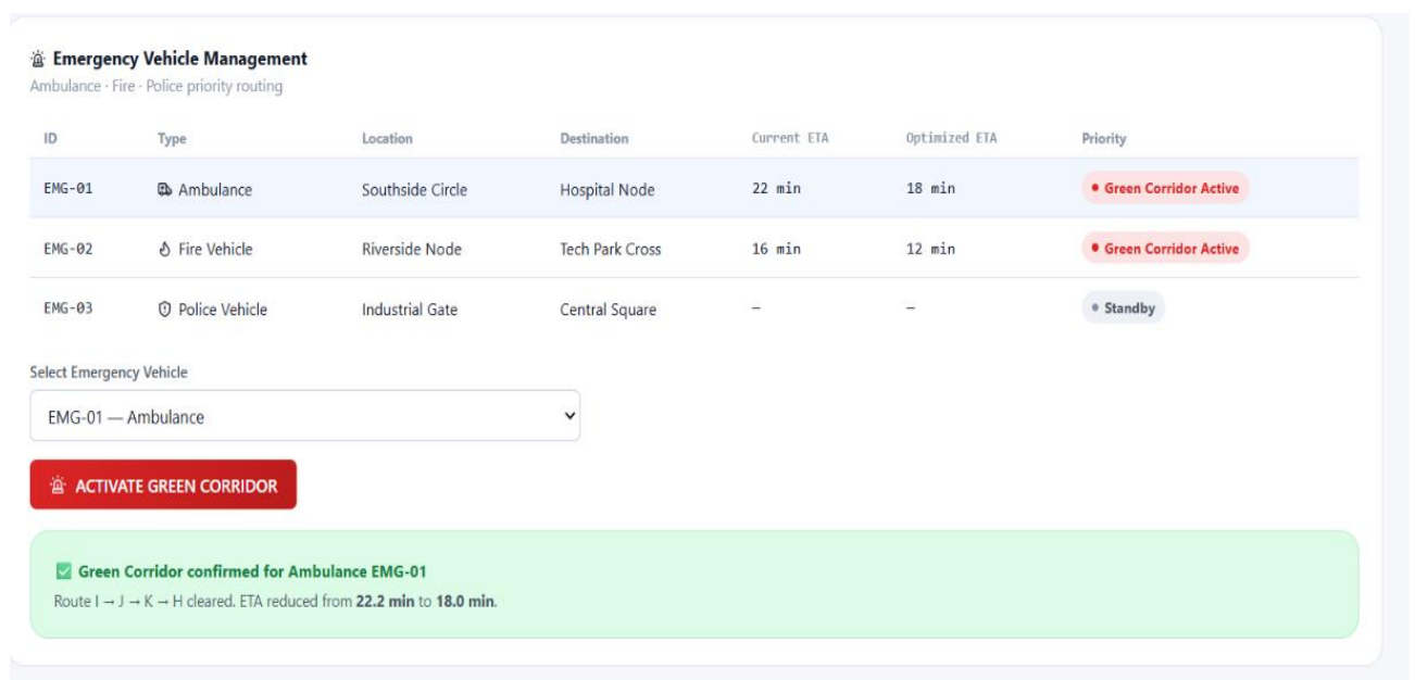
Figure 4. Module 3 Output
