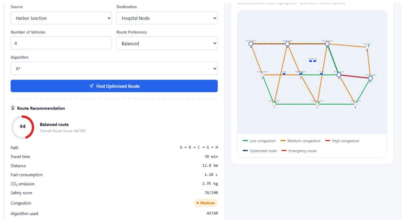
Figure 3. Module 2 Output
