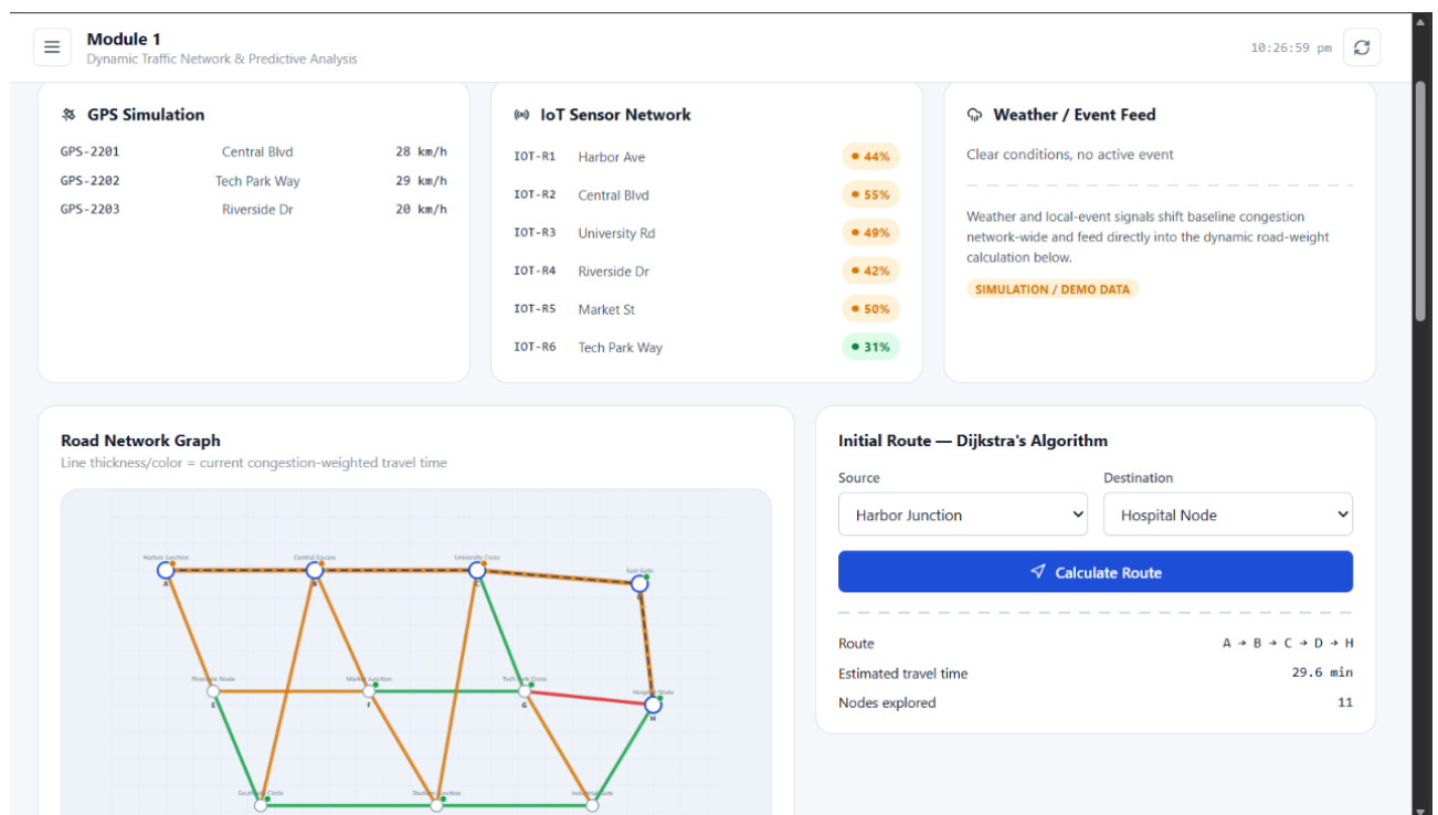
Figure 2. Module 1 Output
