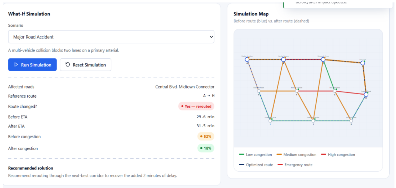
Figure 5. Module 4 Output
